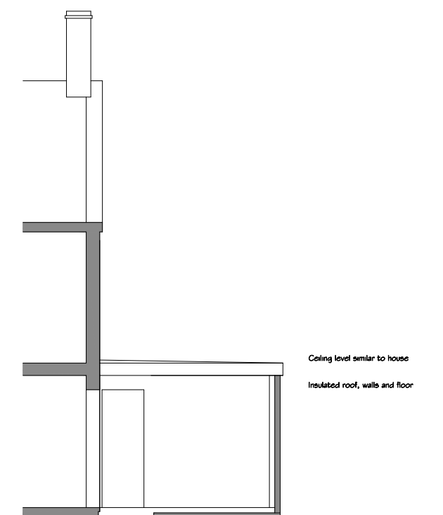
PART SECTION @ 1:100
