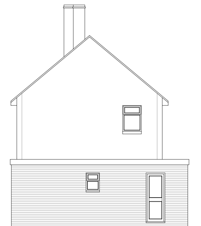
SIDE ELEVATION @ 1:100
